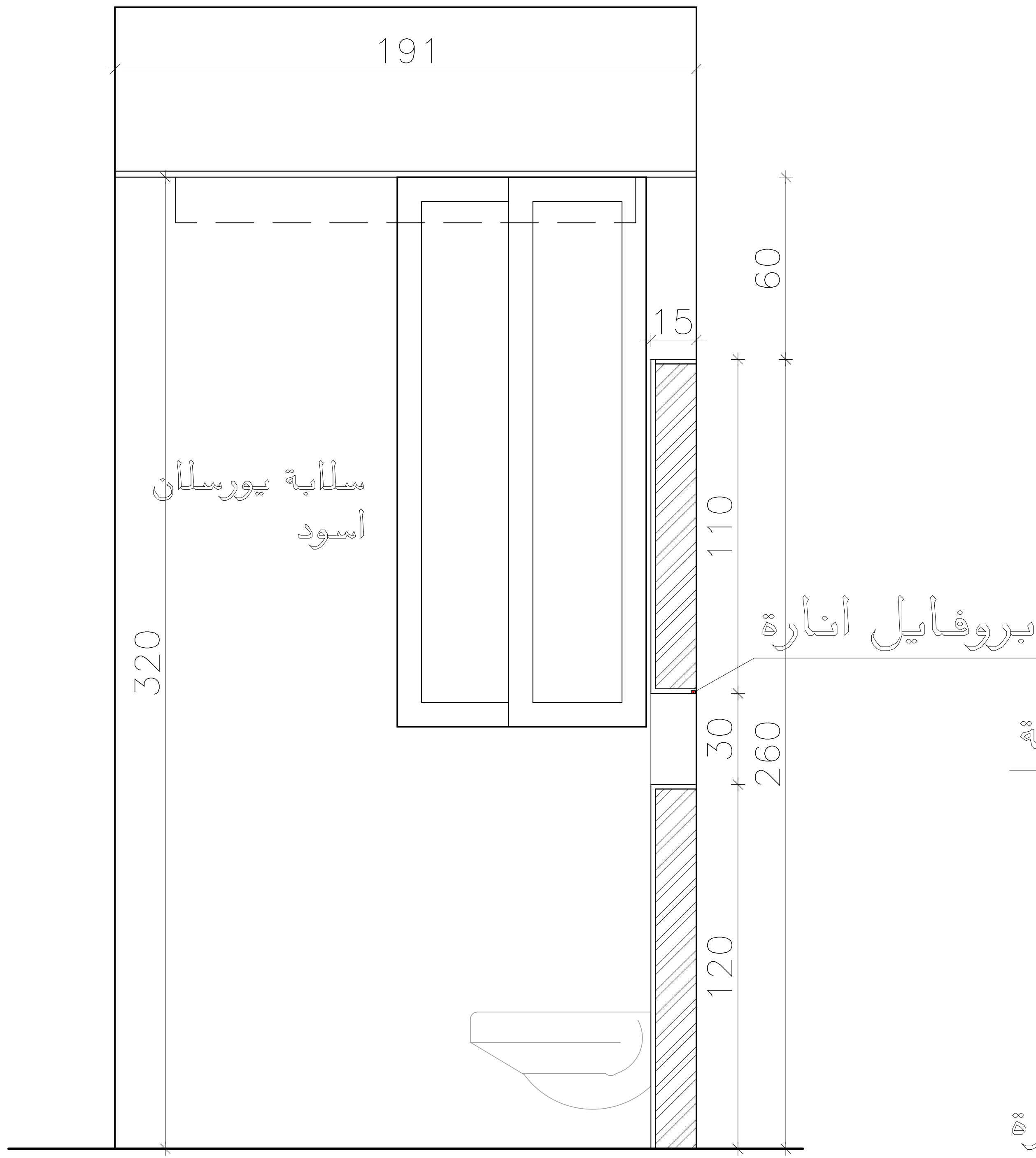
Elevation (C)
