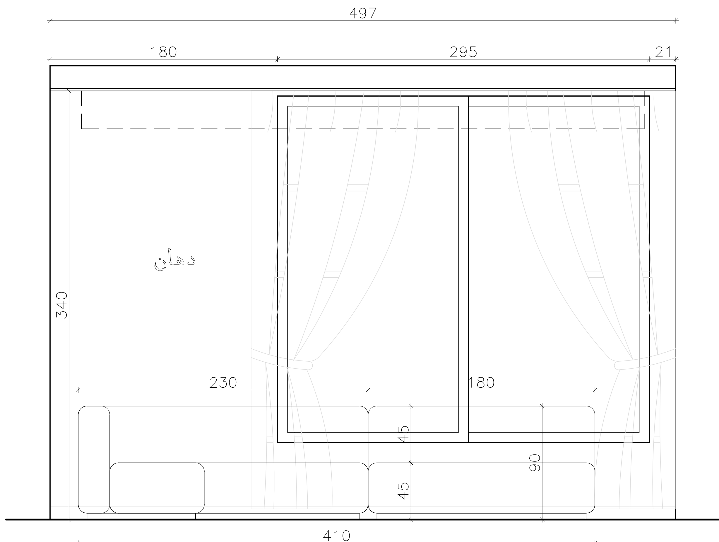
Elevation (A)
