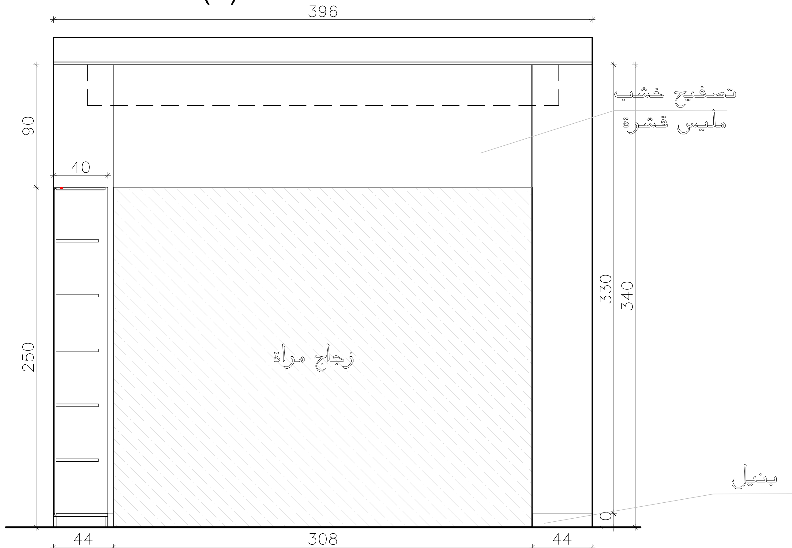
Elevation (B)
