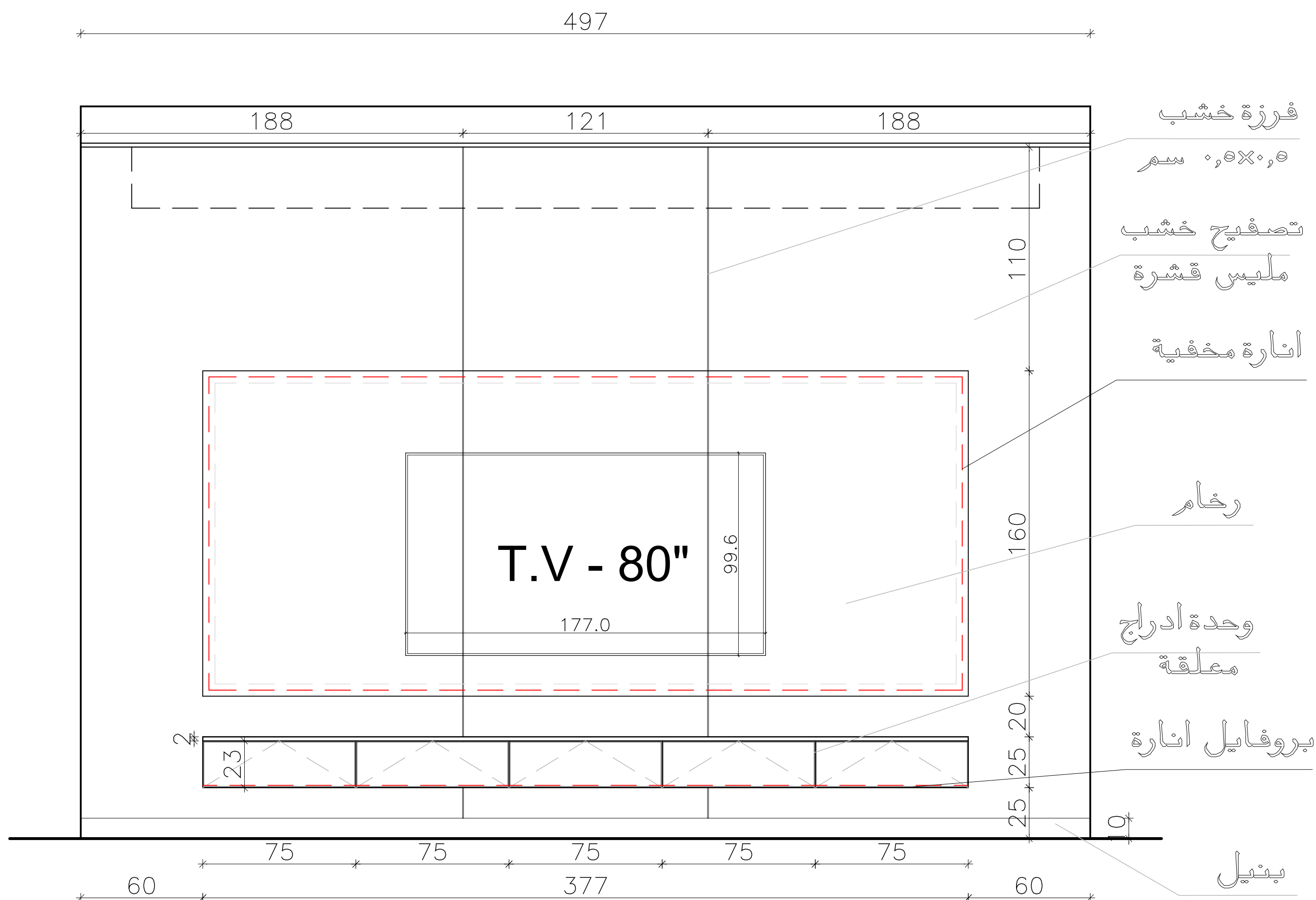
Elevation (C)
