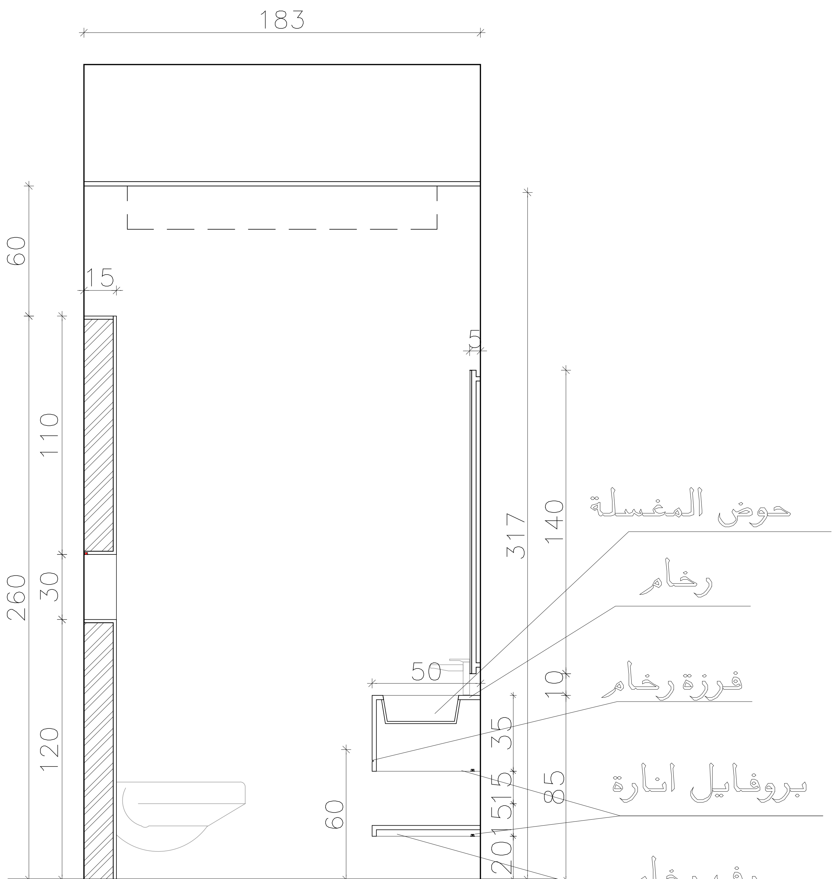
Elevation (C)
