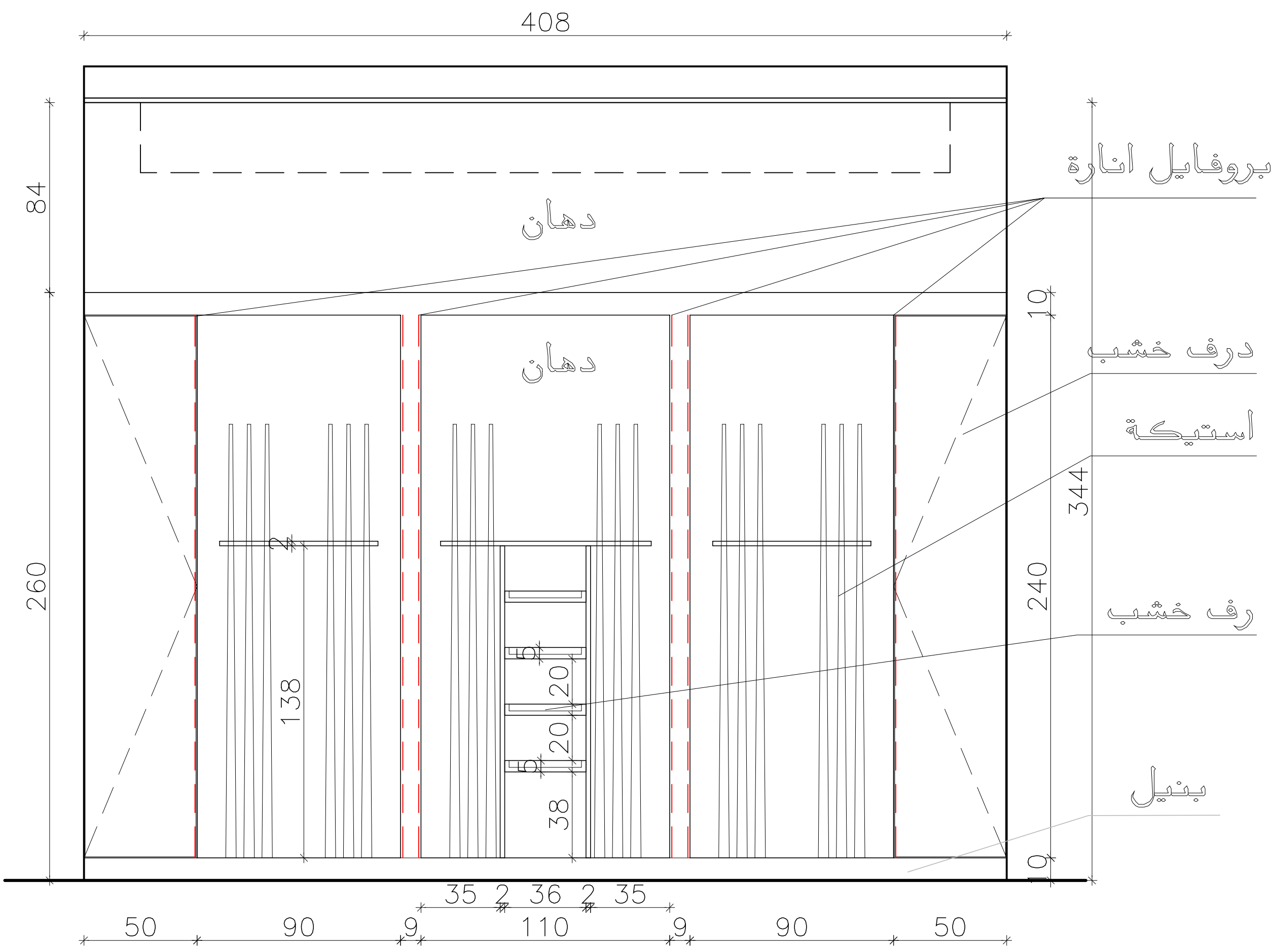
Elevation (A)
