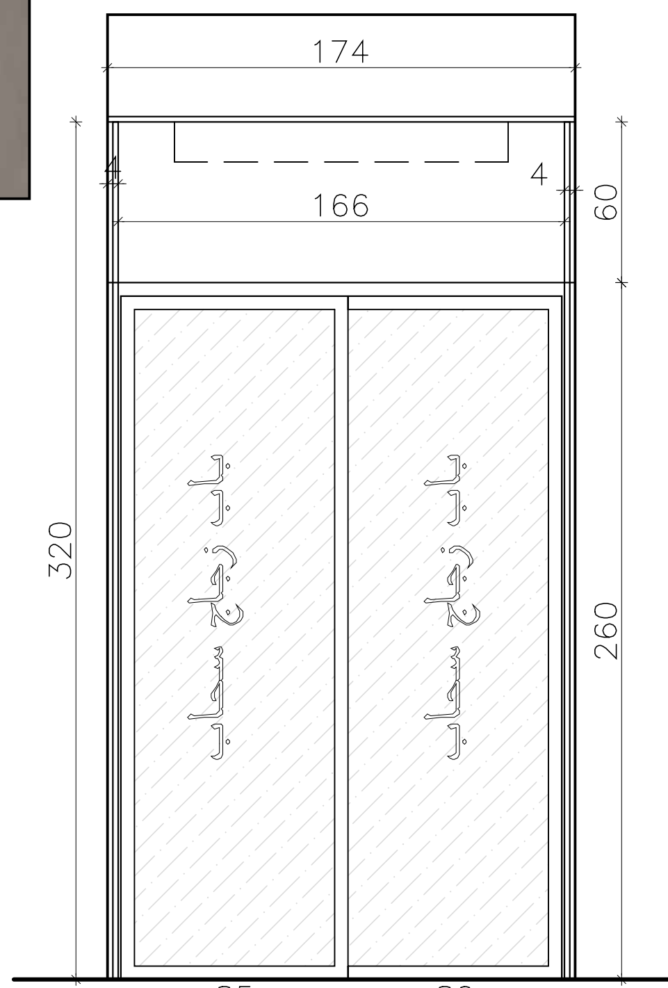
Elevation (A)
