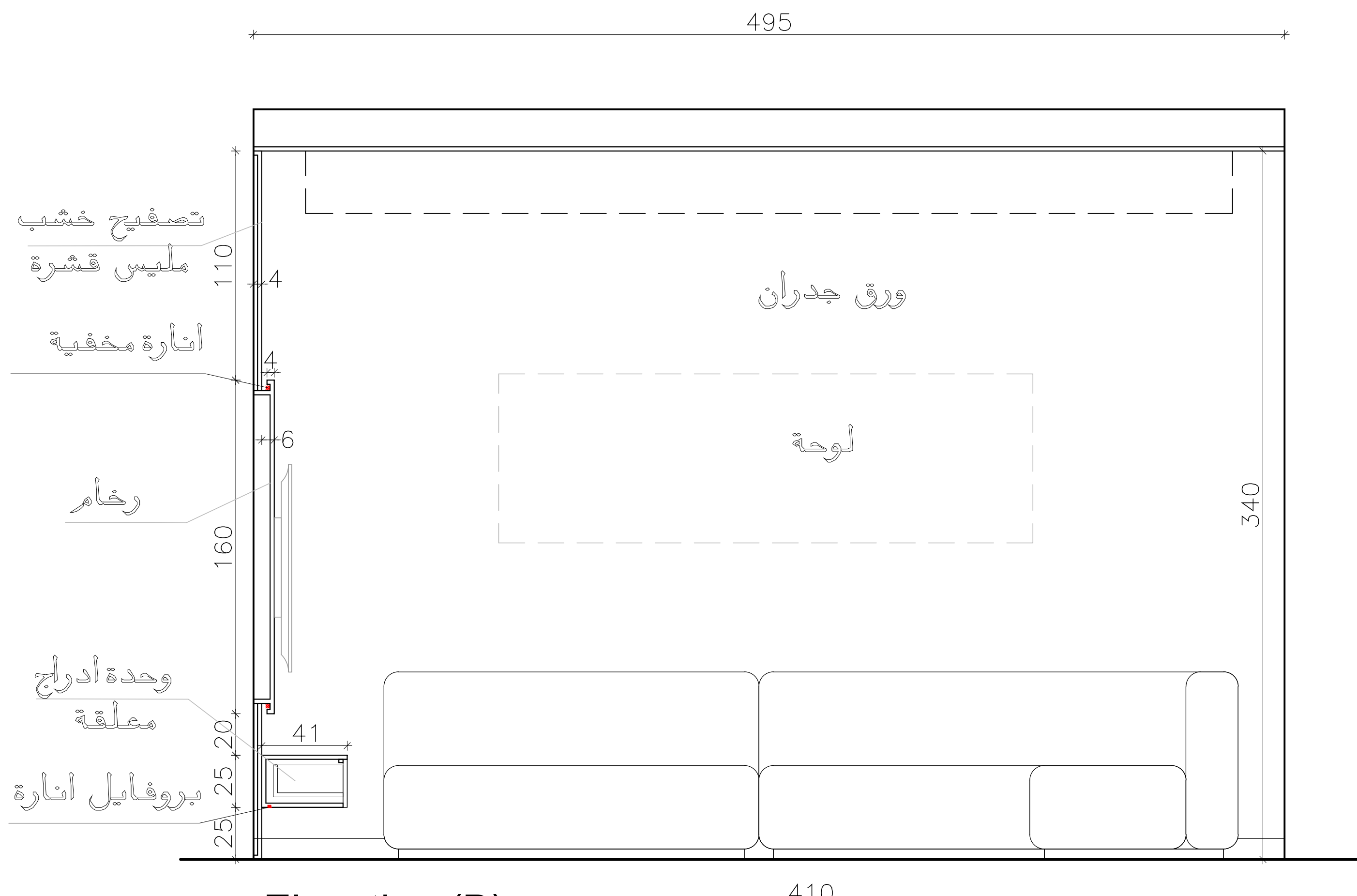
Elevation (B)
