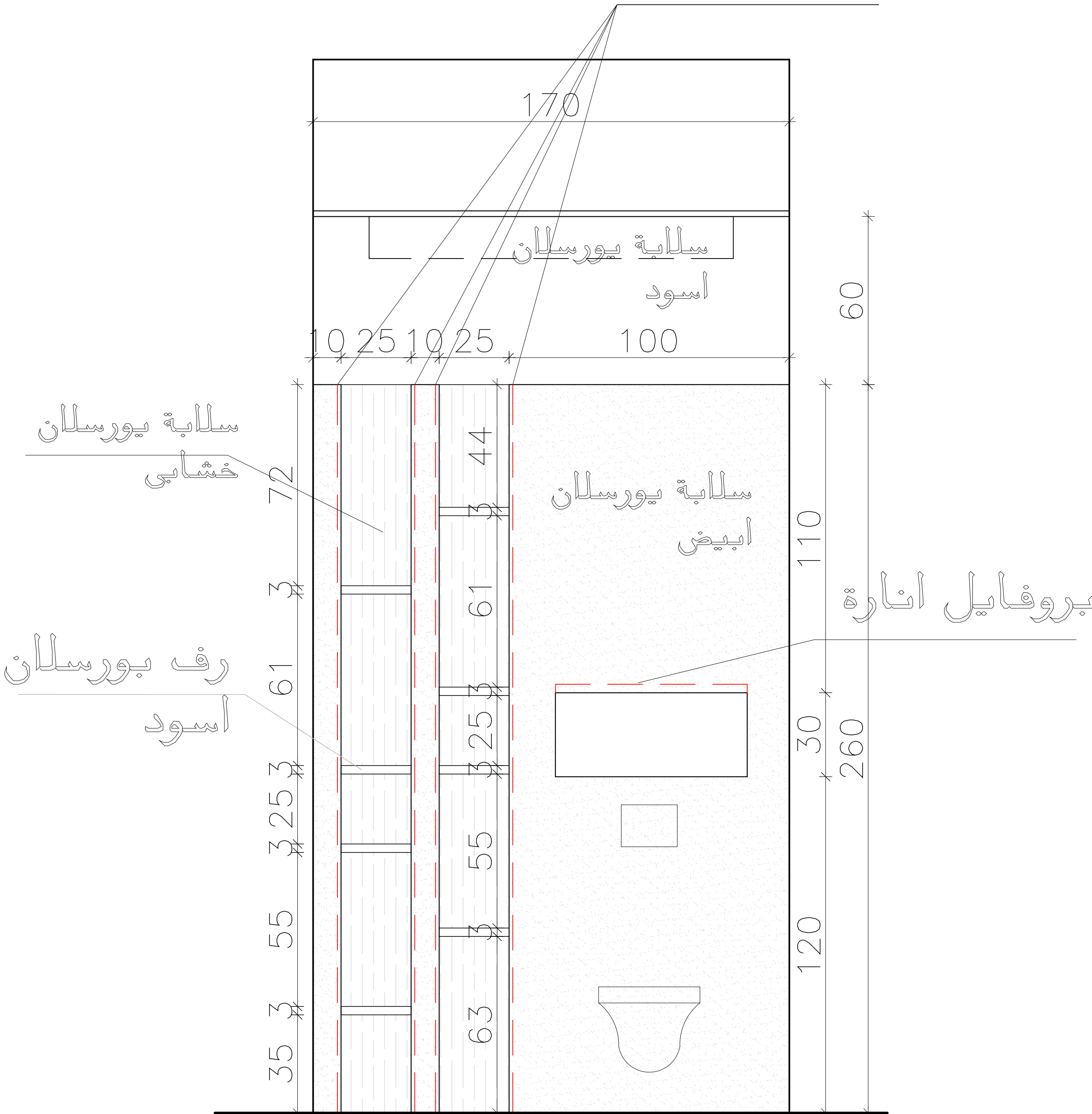
Elevation (B)
