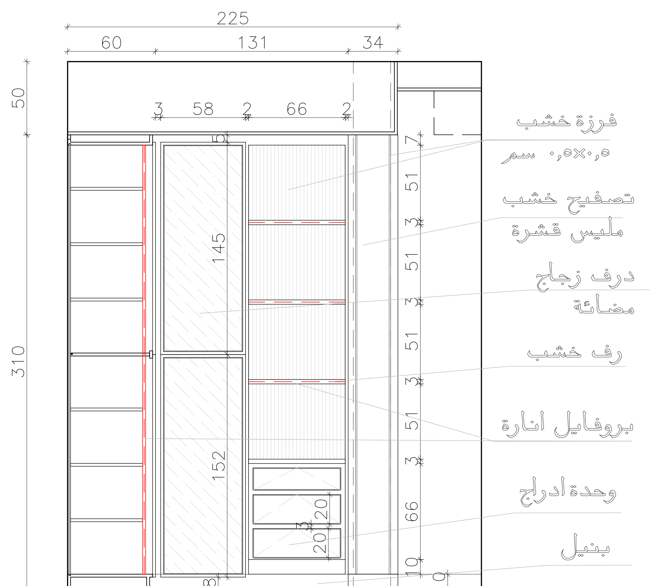
Elevation (B)
