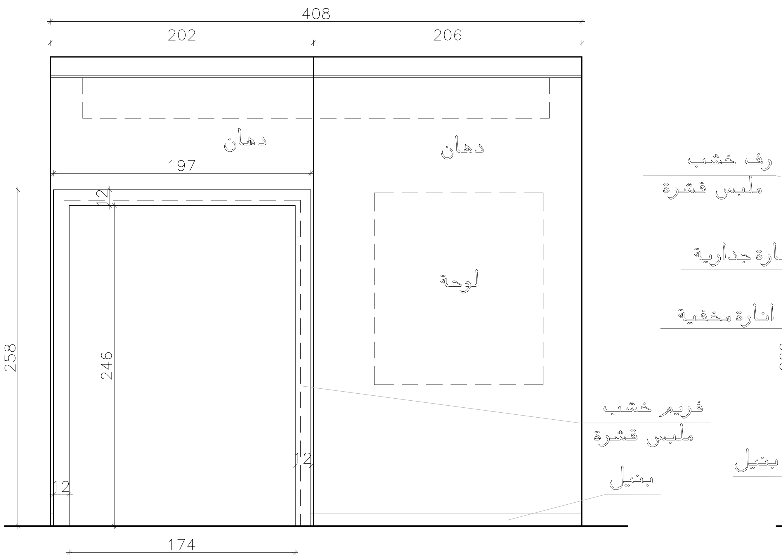
Elevation (C)
