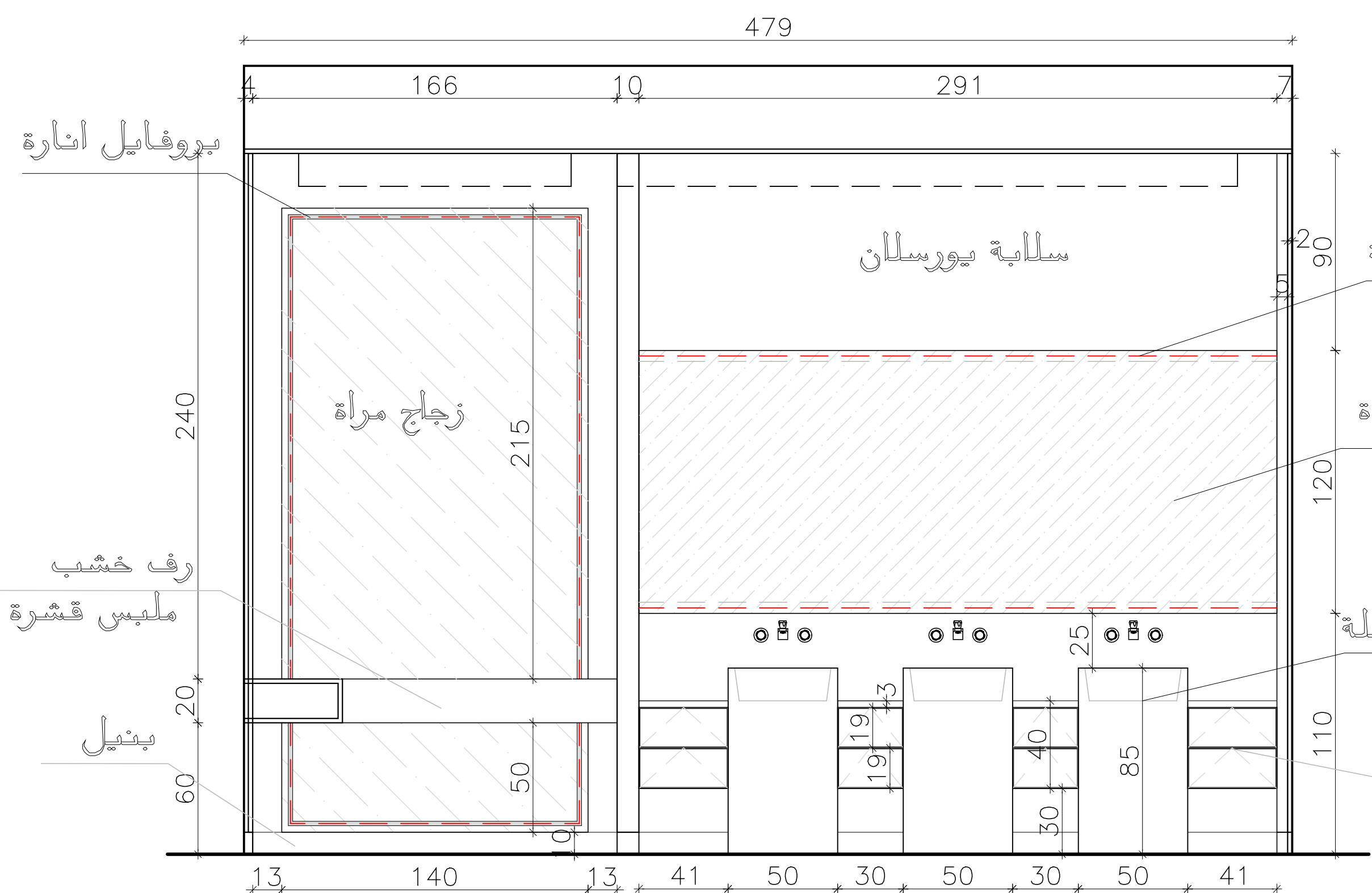
Elevation (C)
