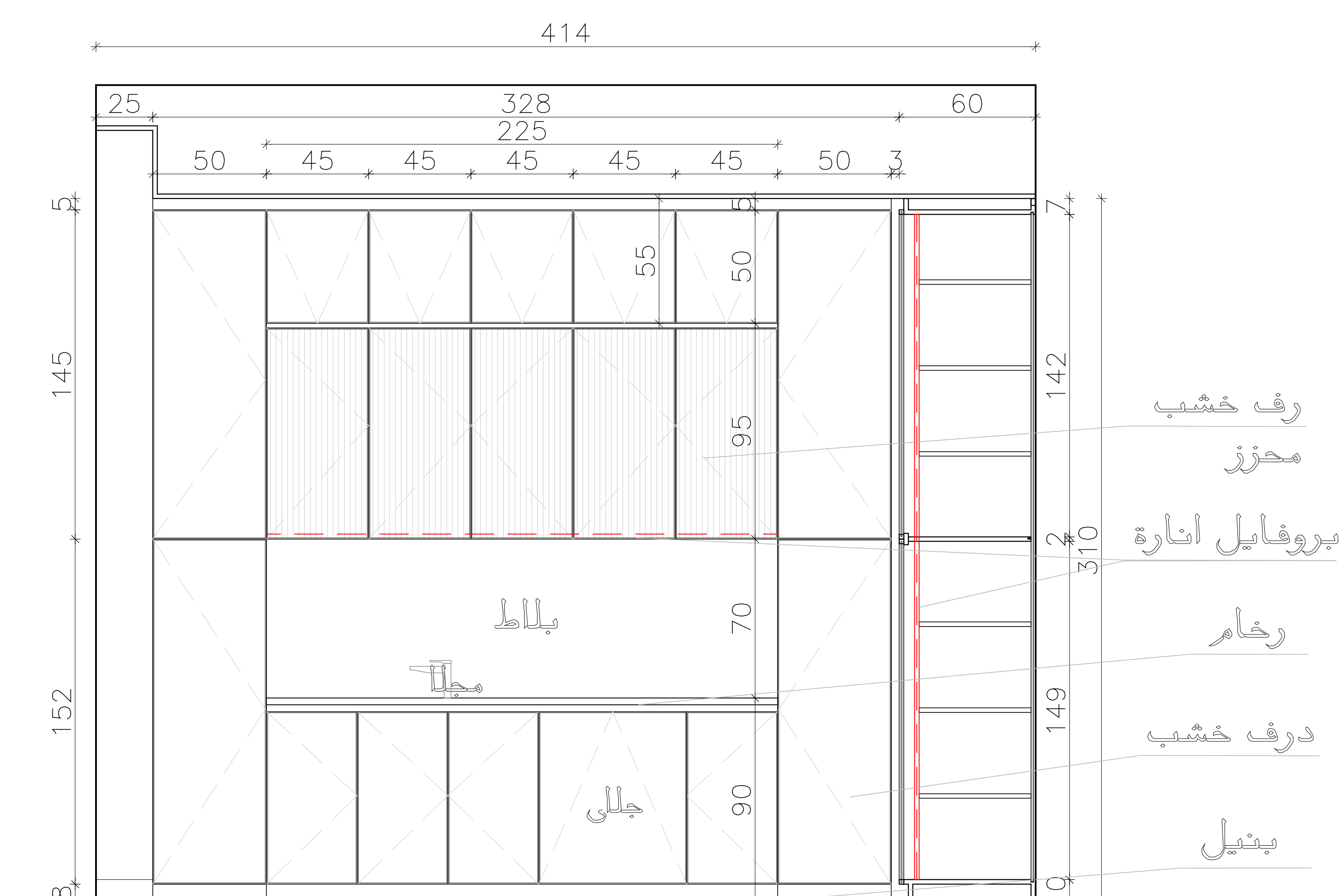
Elevation (C)
