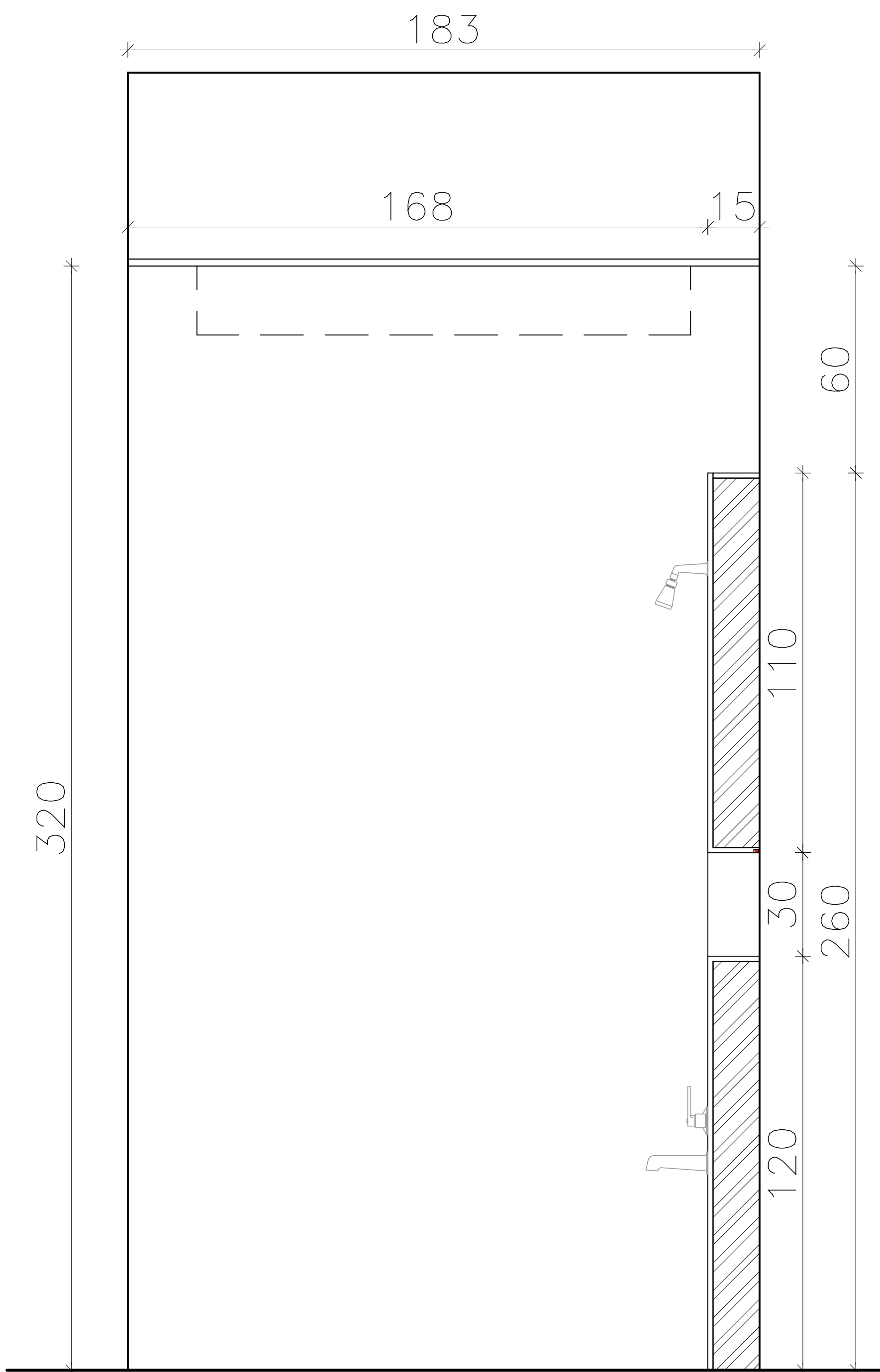
Elevation (A)
