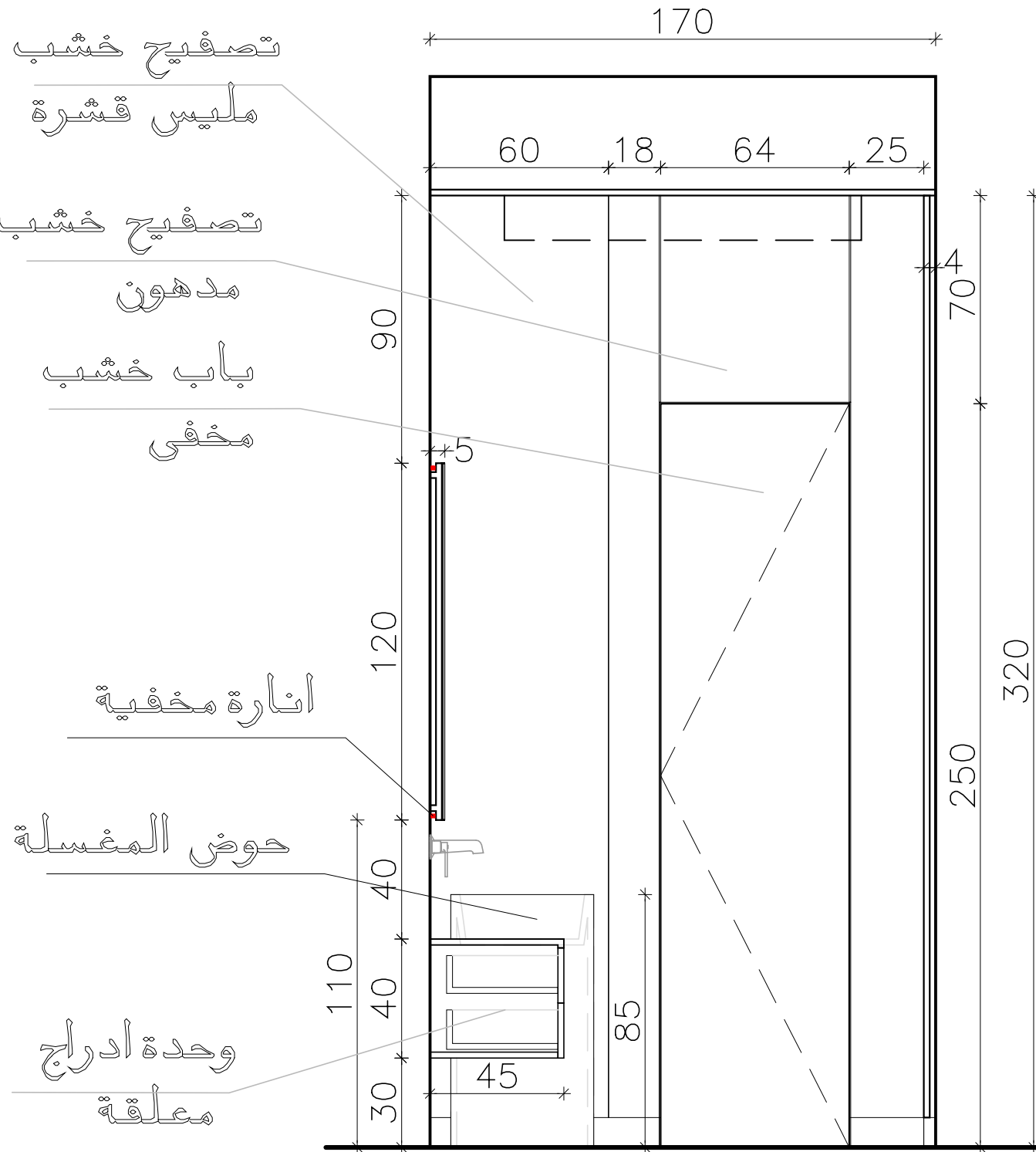
Elevation (F)
