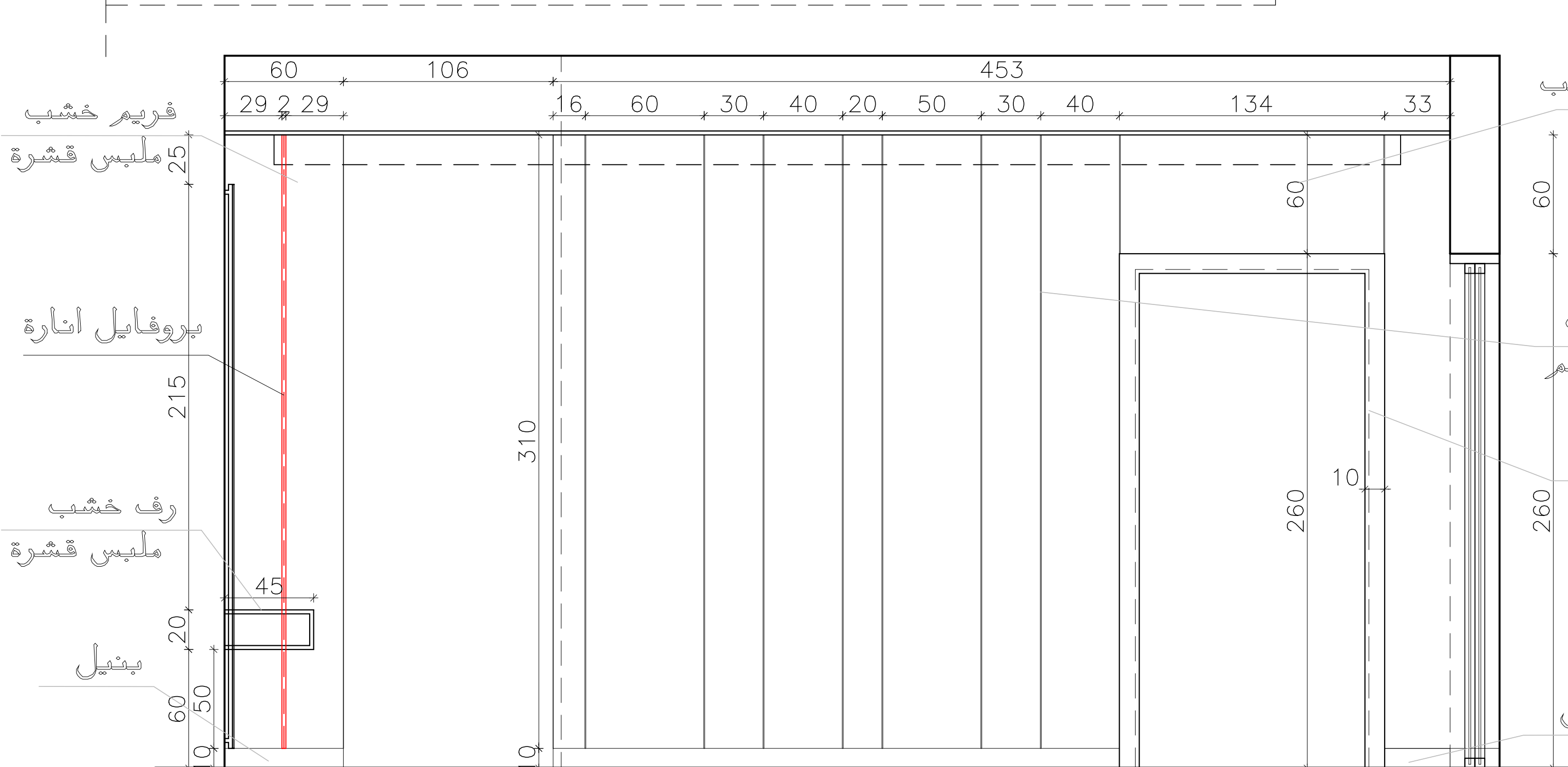
Elevation (B)
