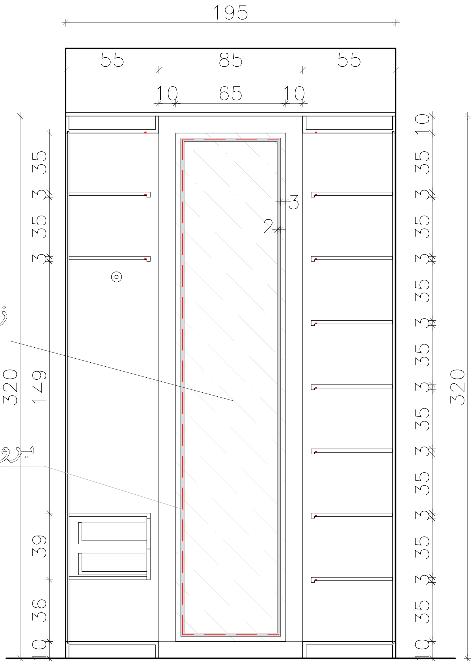
Elevation (B)
