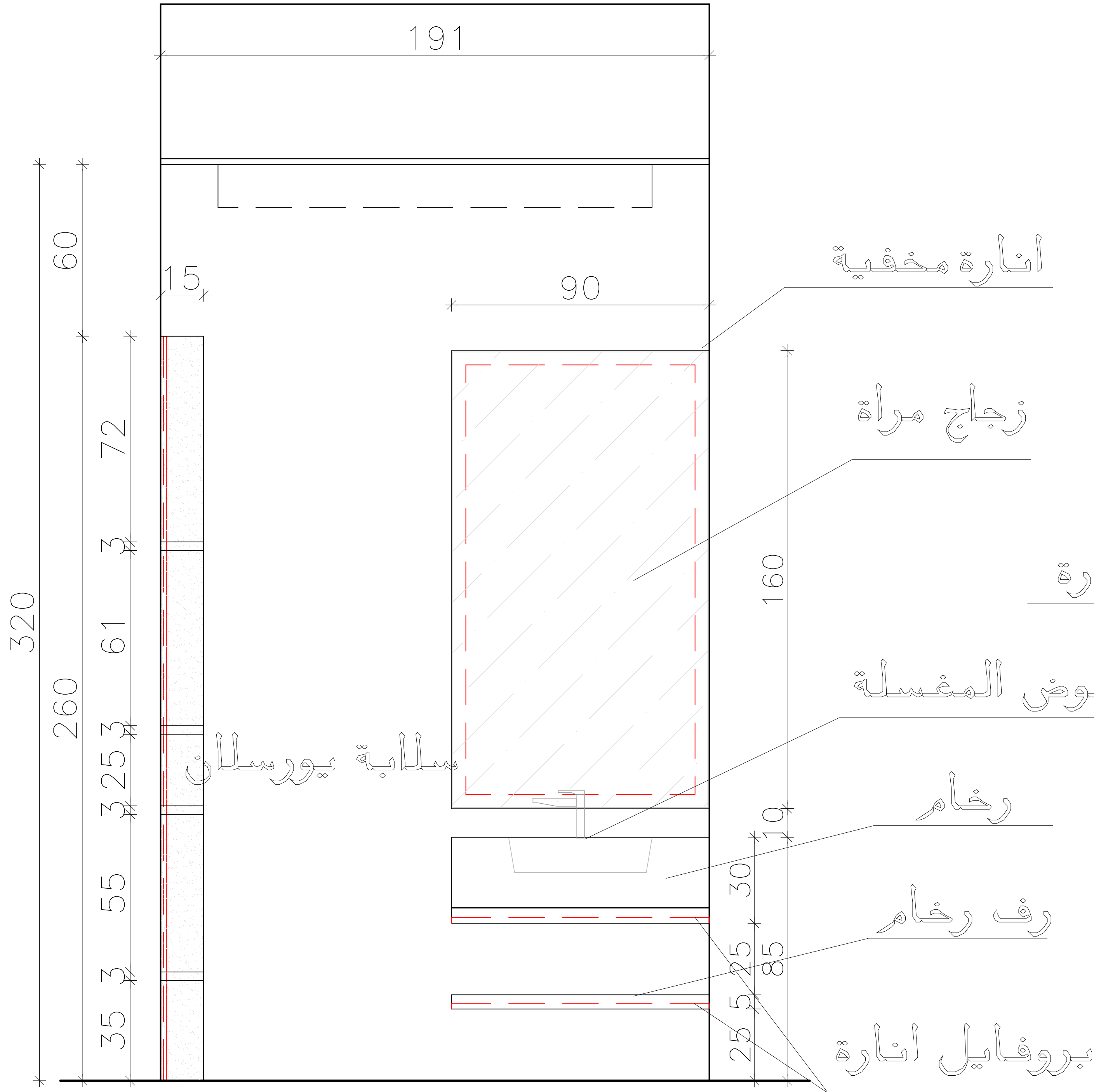
Elevation (A)
