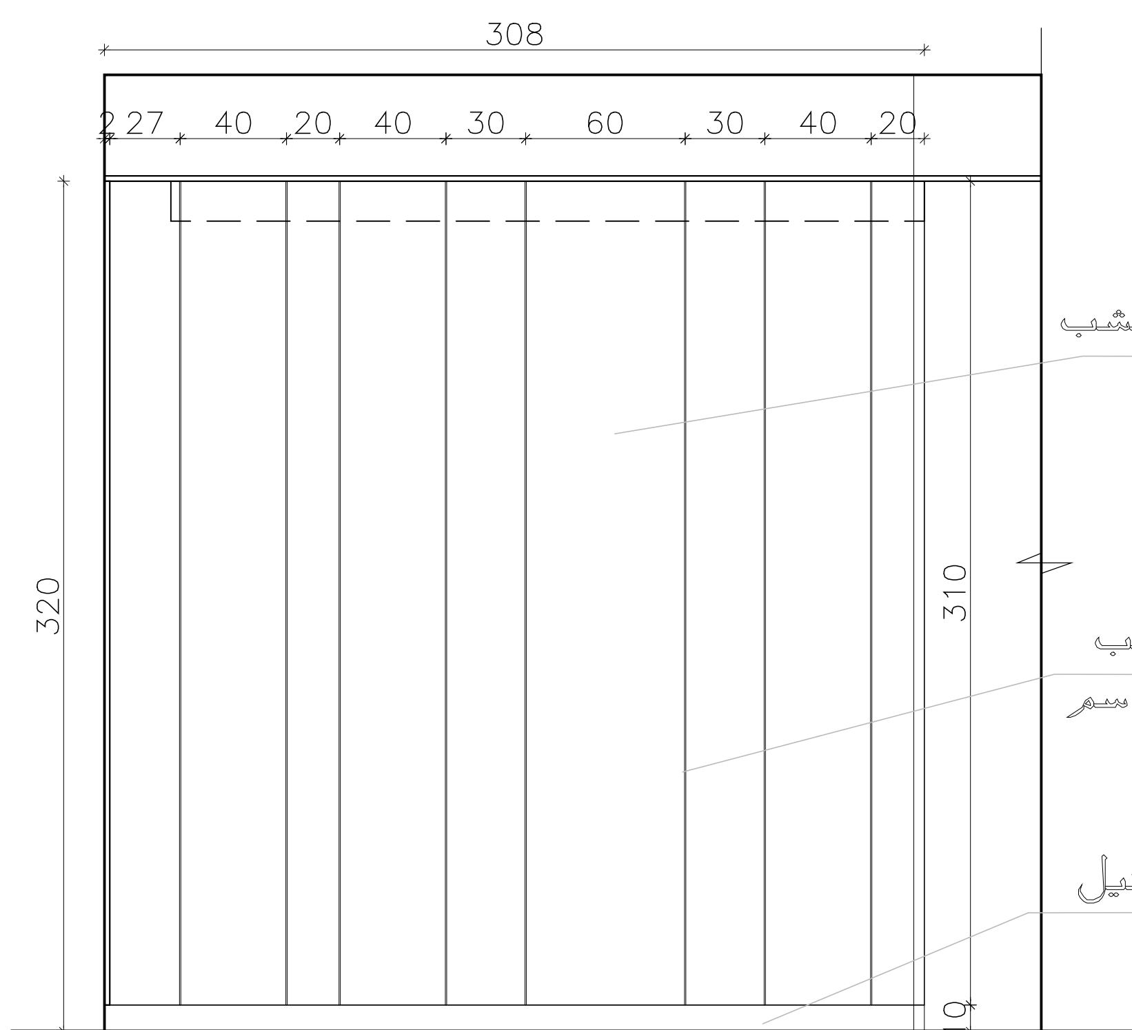
Elevation (E)
