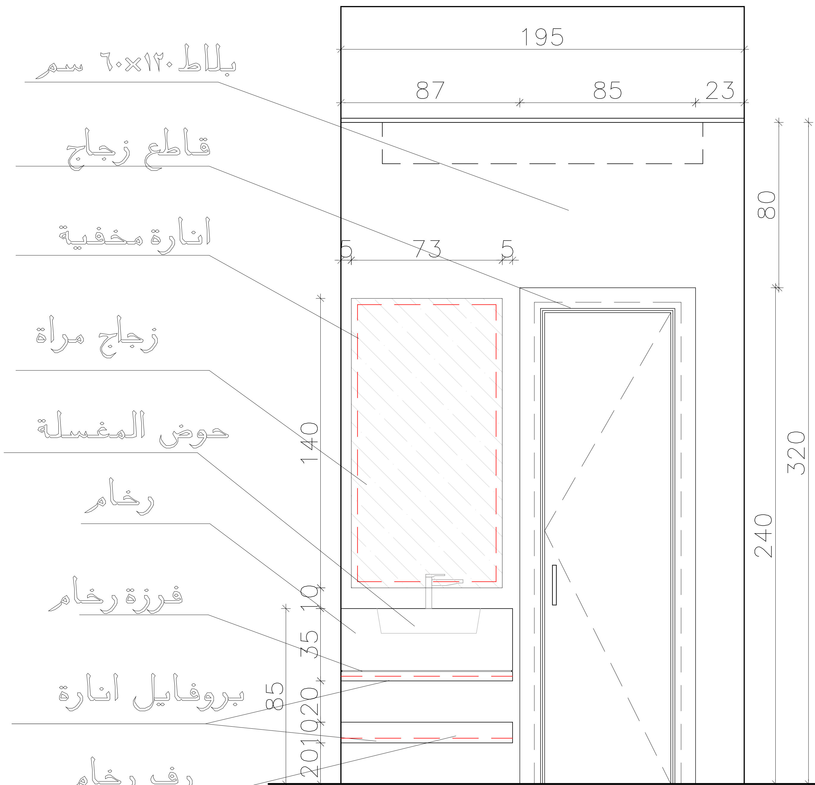
Elevation (B)
