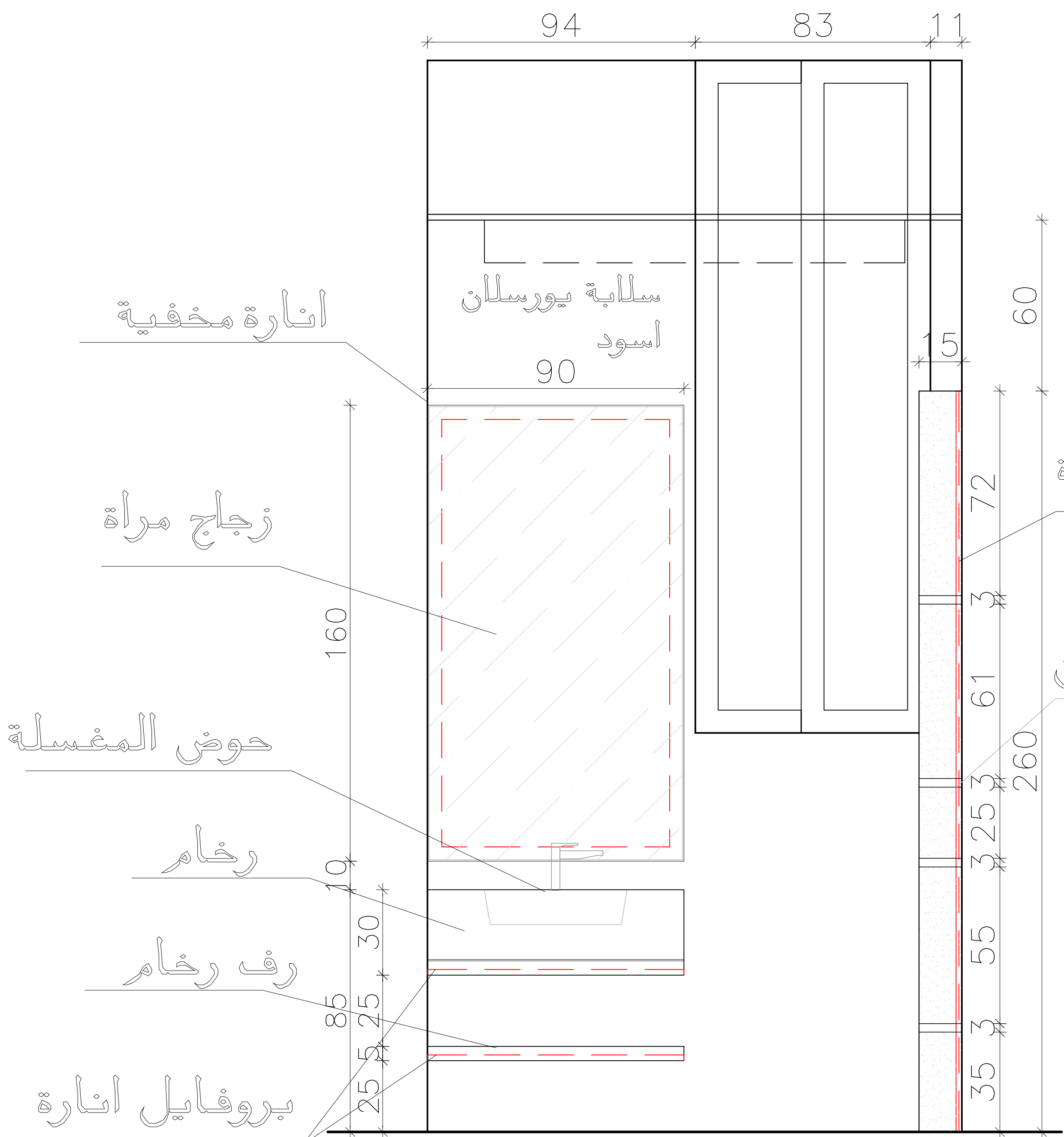
Elevation (C)
