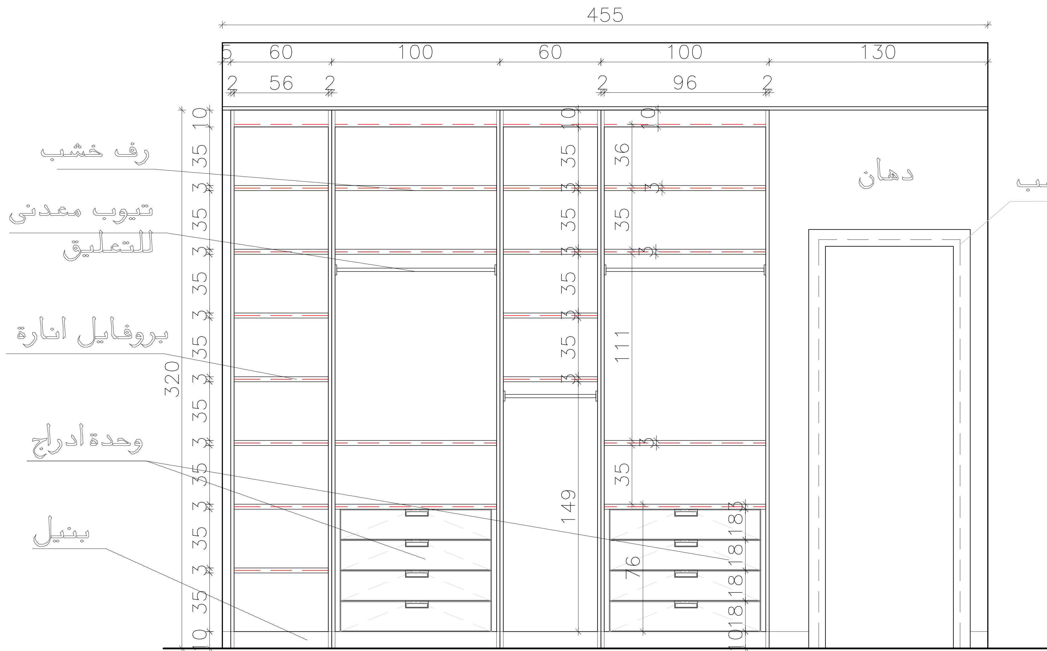
Elevation (A)
