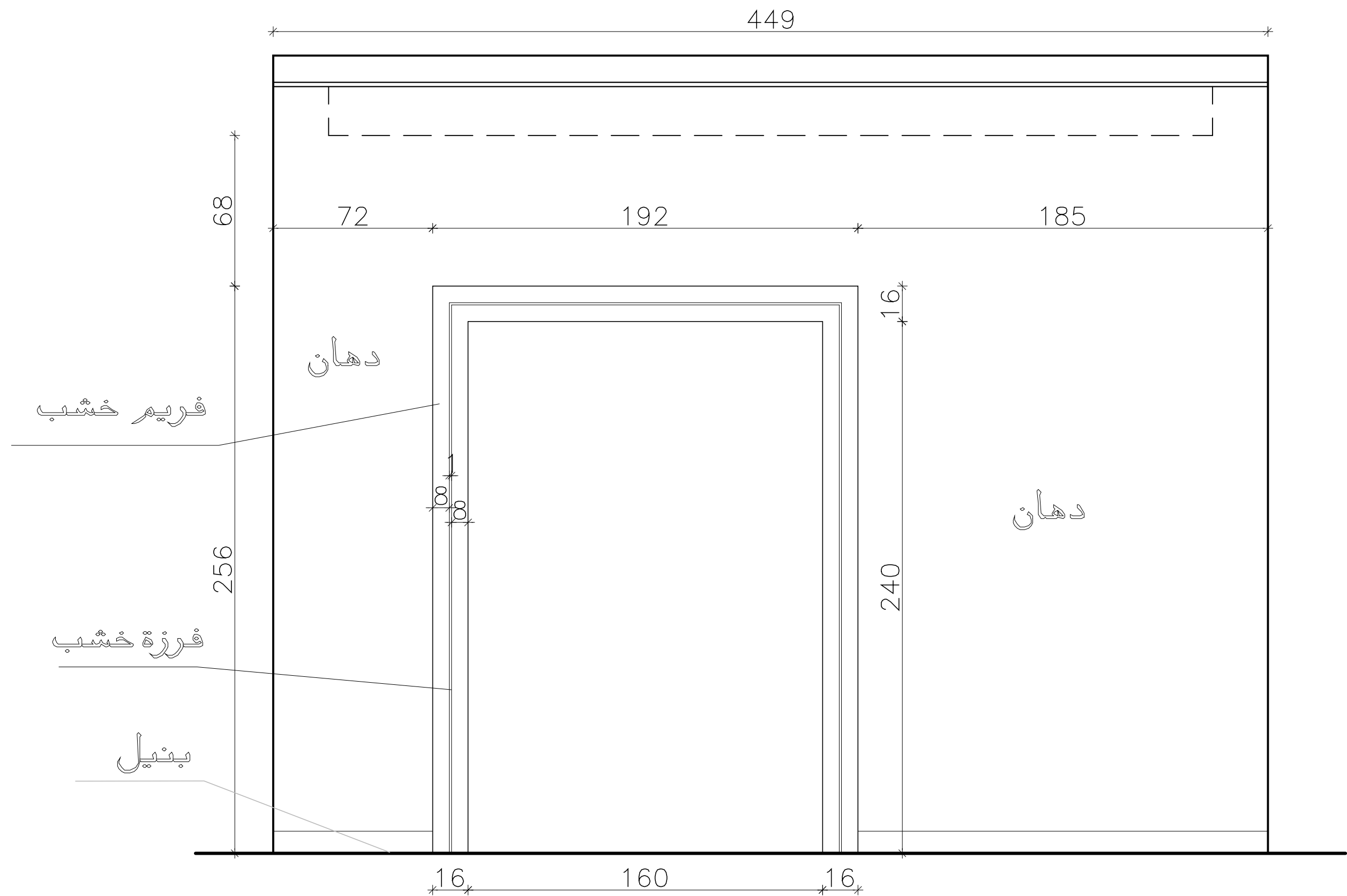
Elevation (A)
