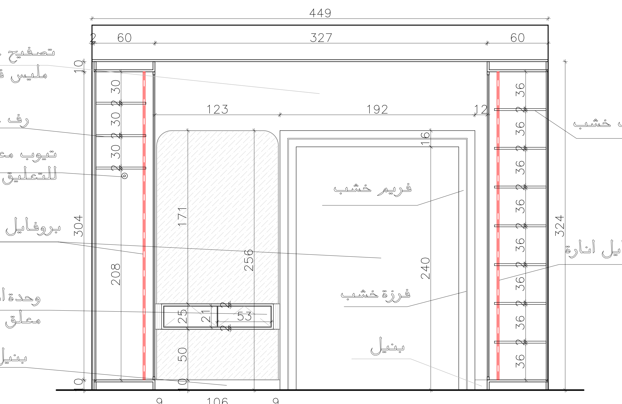
Elevation (C)
