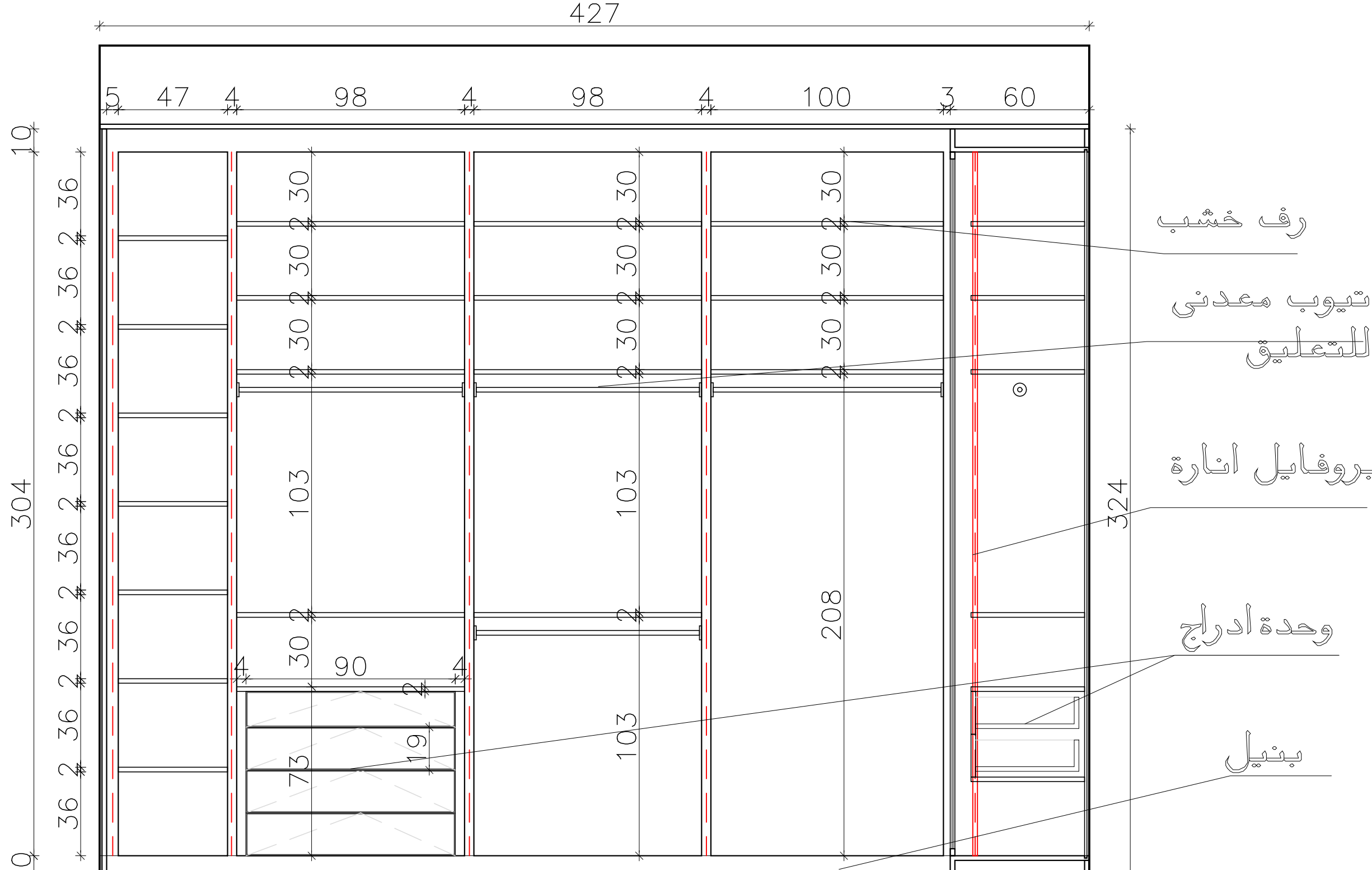
Elevation (B)
