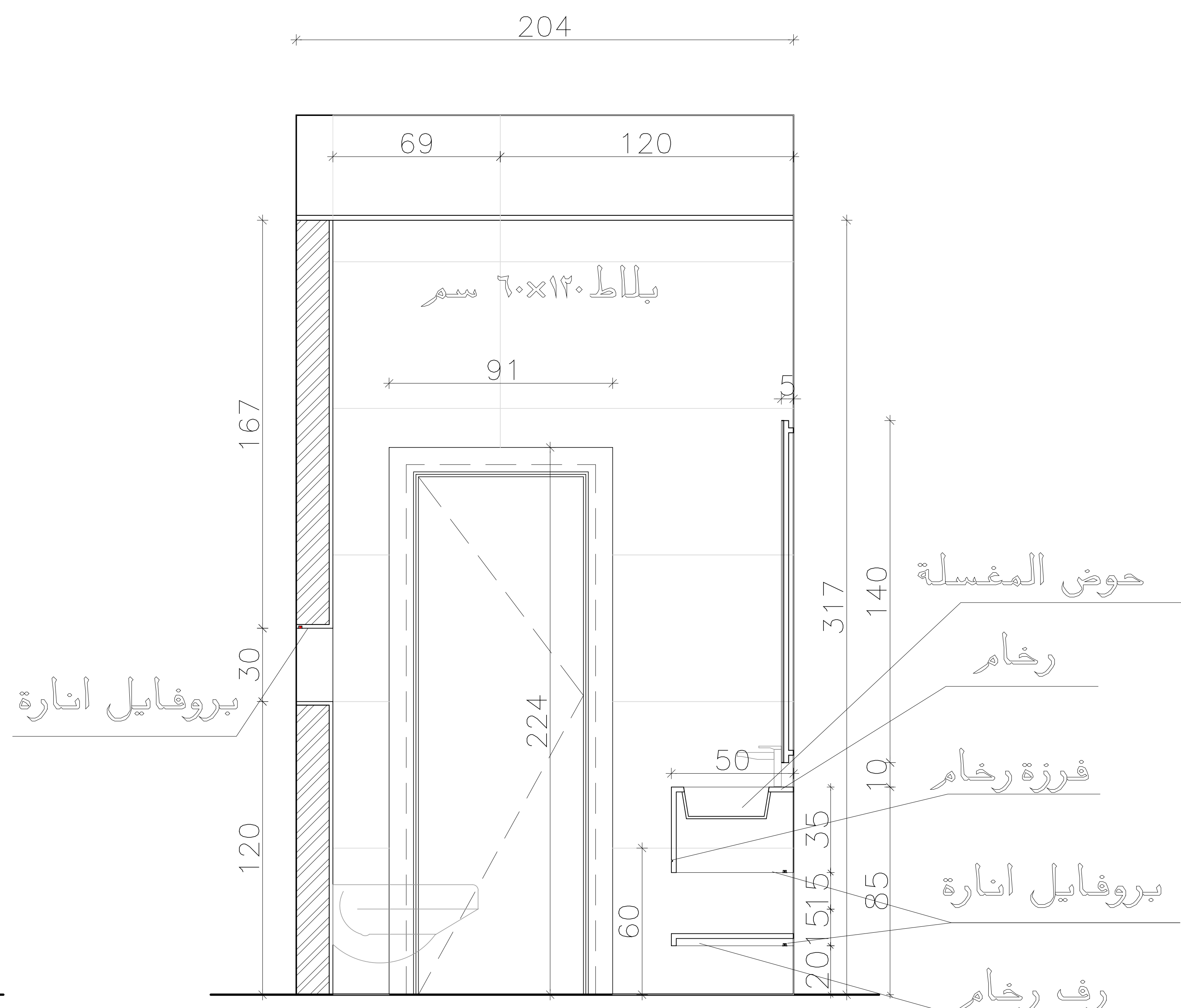
Elevation (B)
