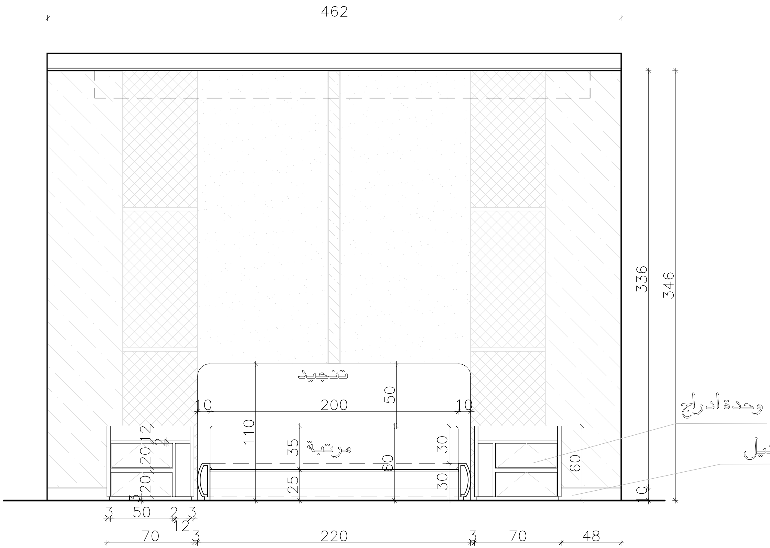
Elevation (C)
