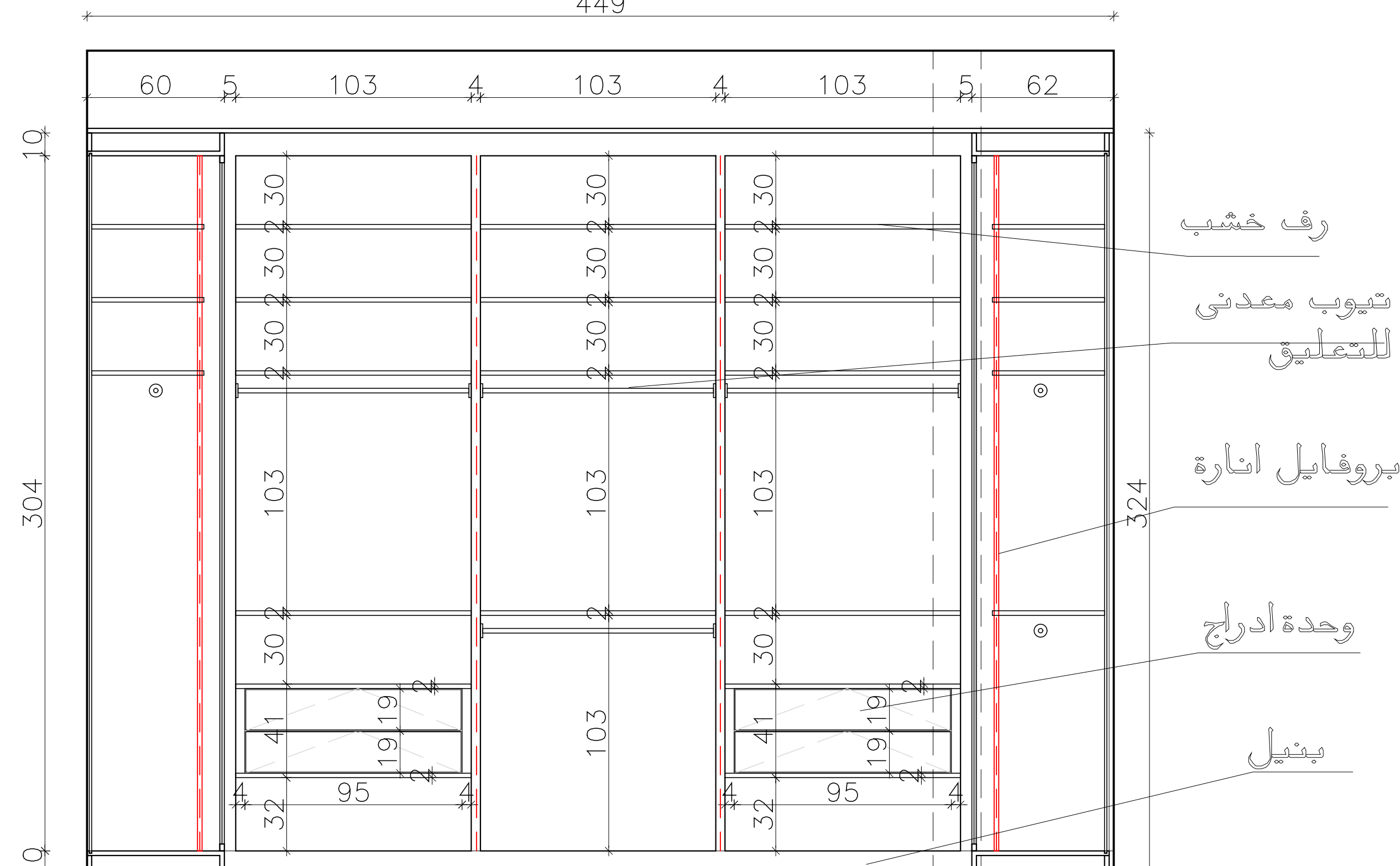
Elevation (A)
