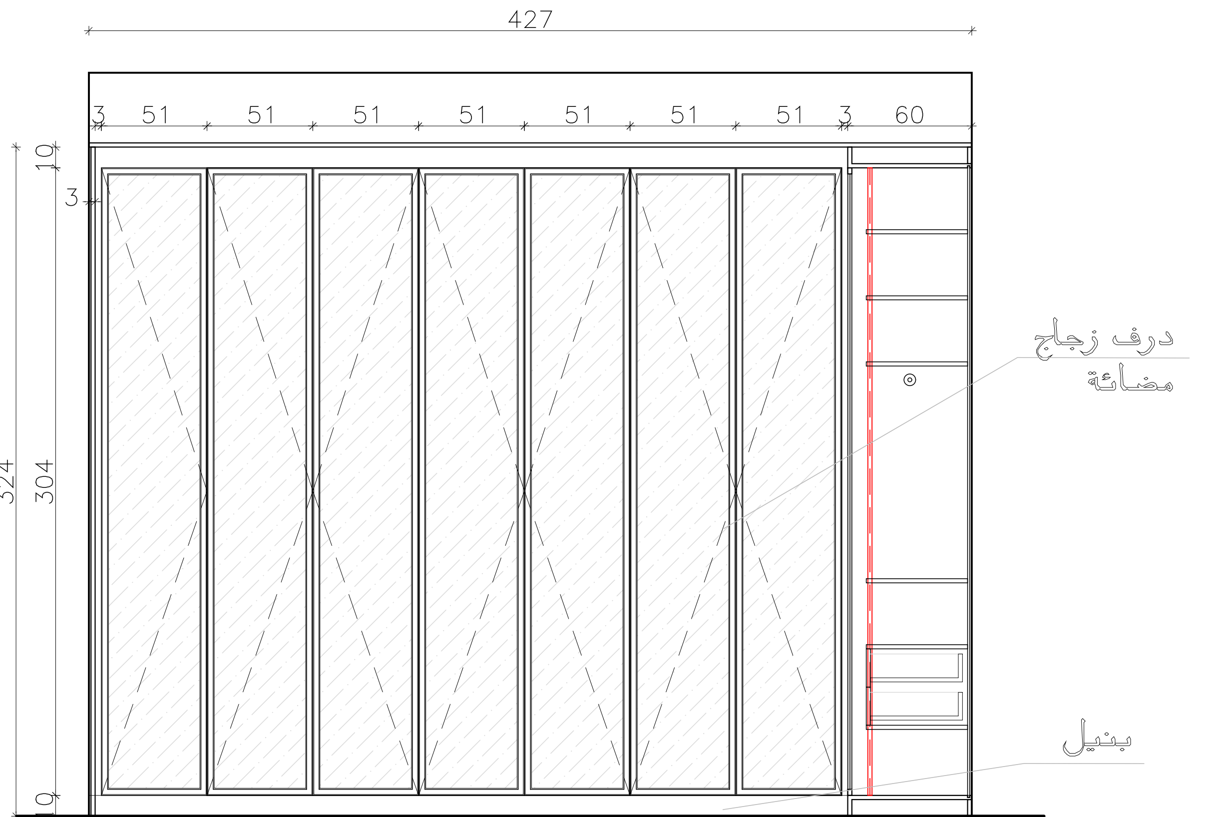
Elevation (B)
