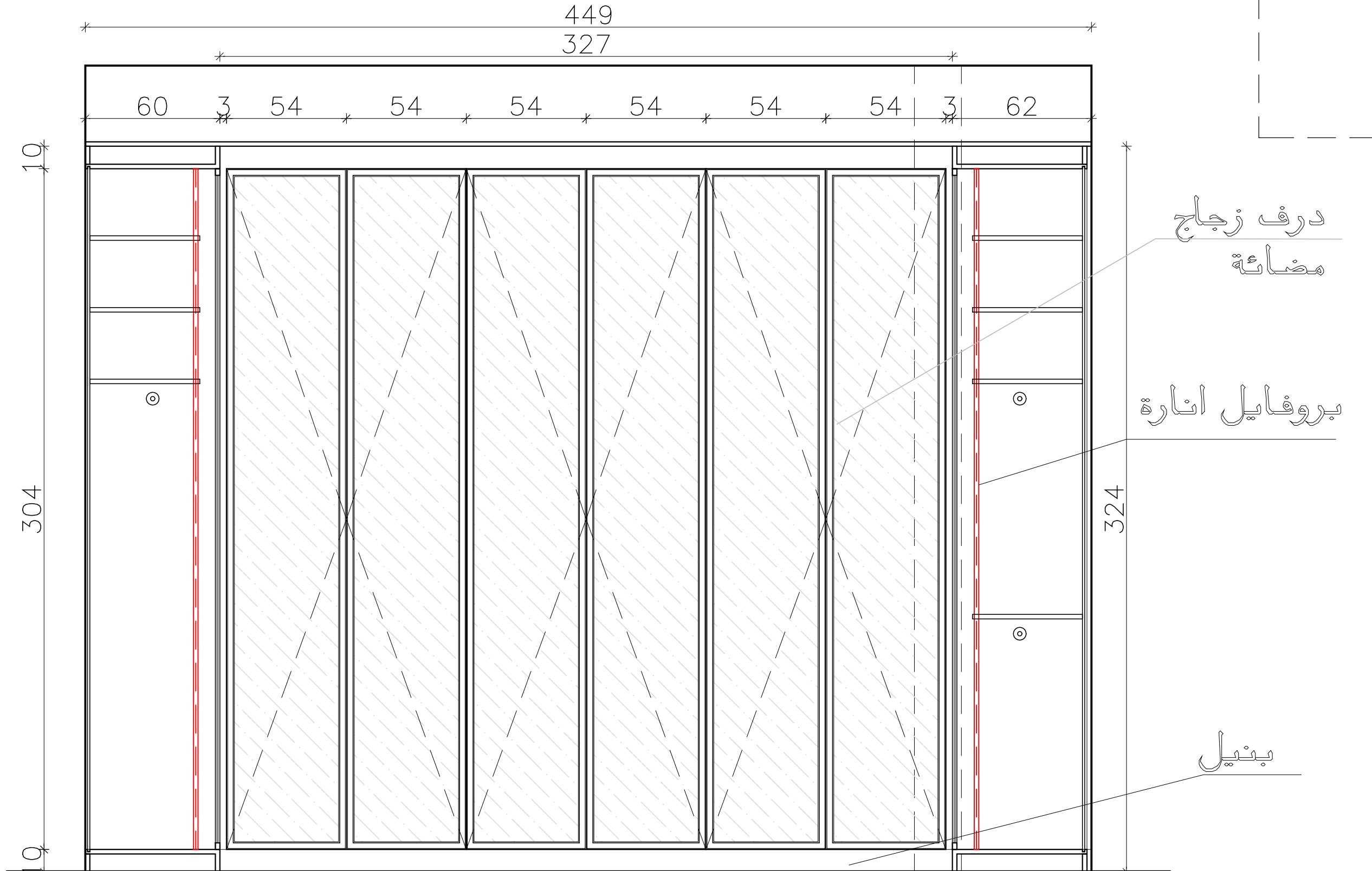
Elevation (A)
