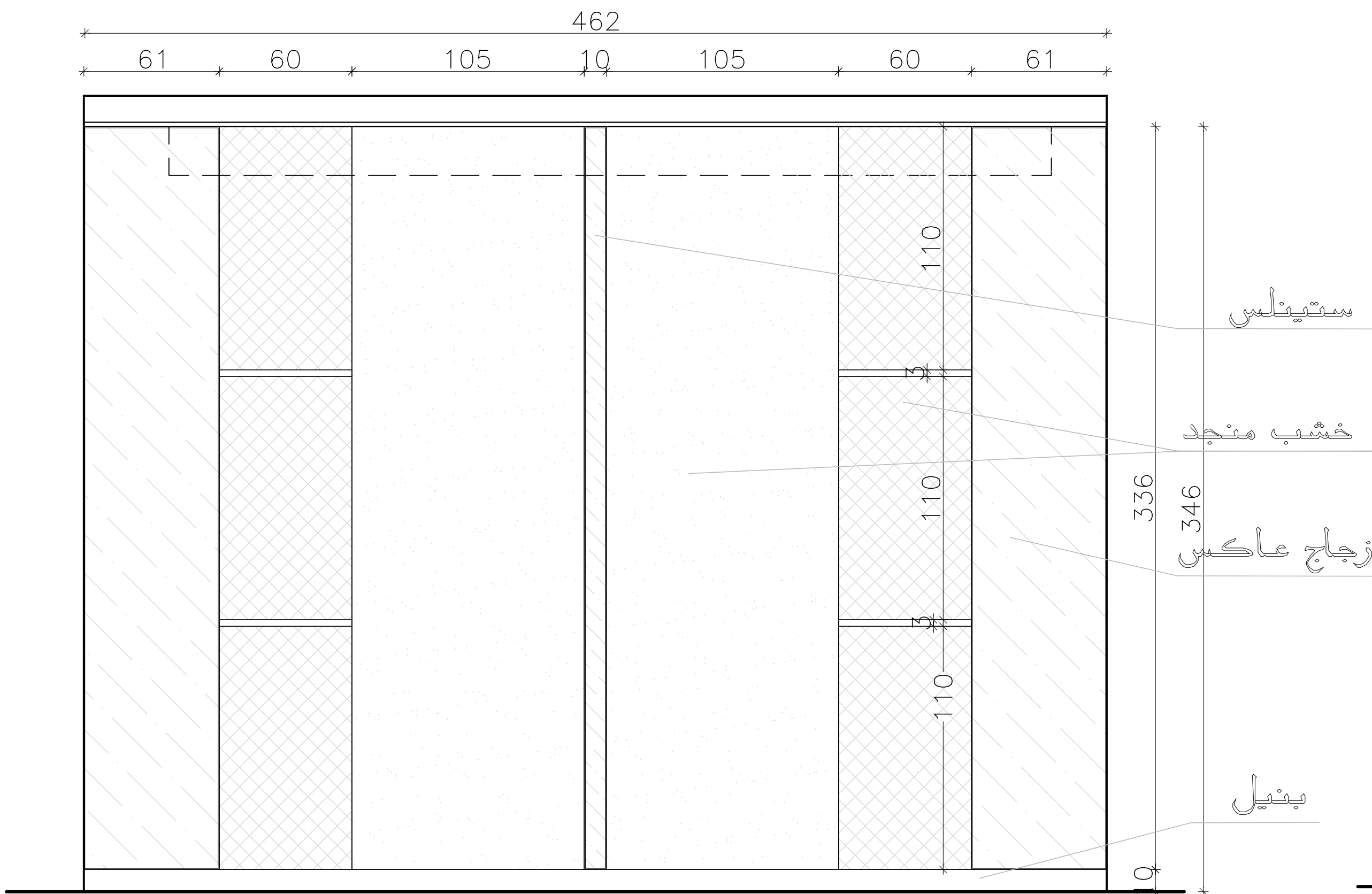
Elevation (C)
