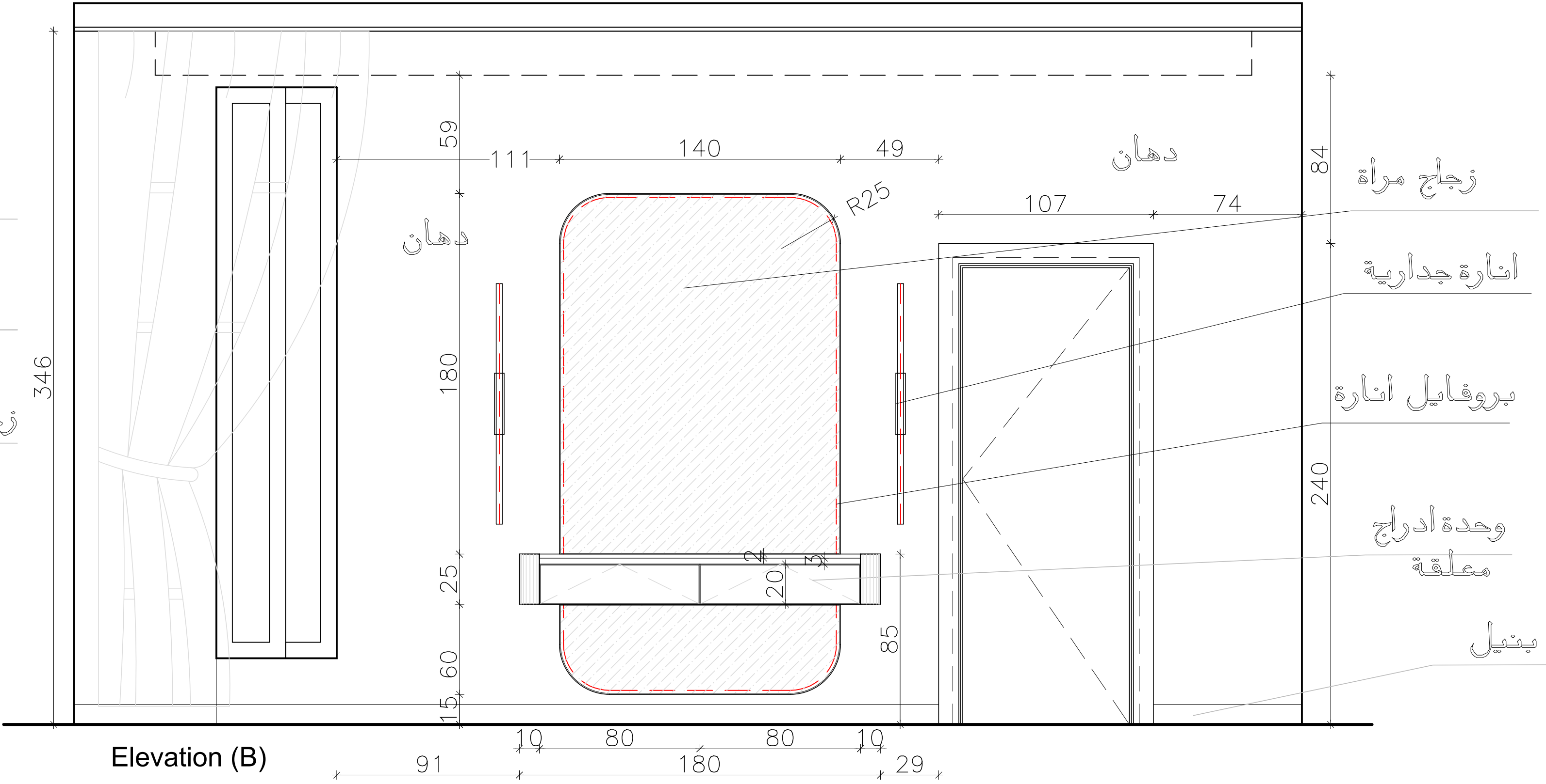
Elevation (B)
