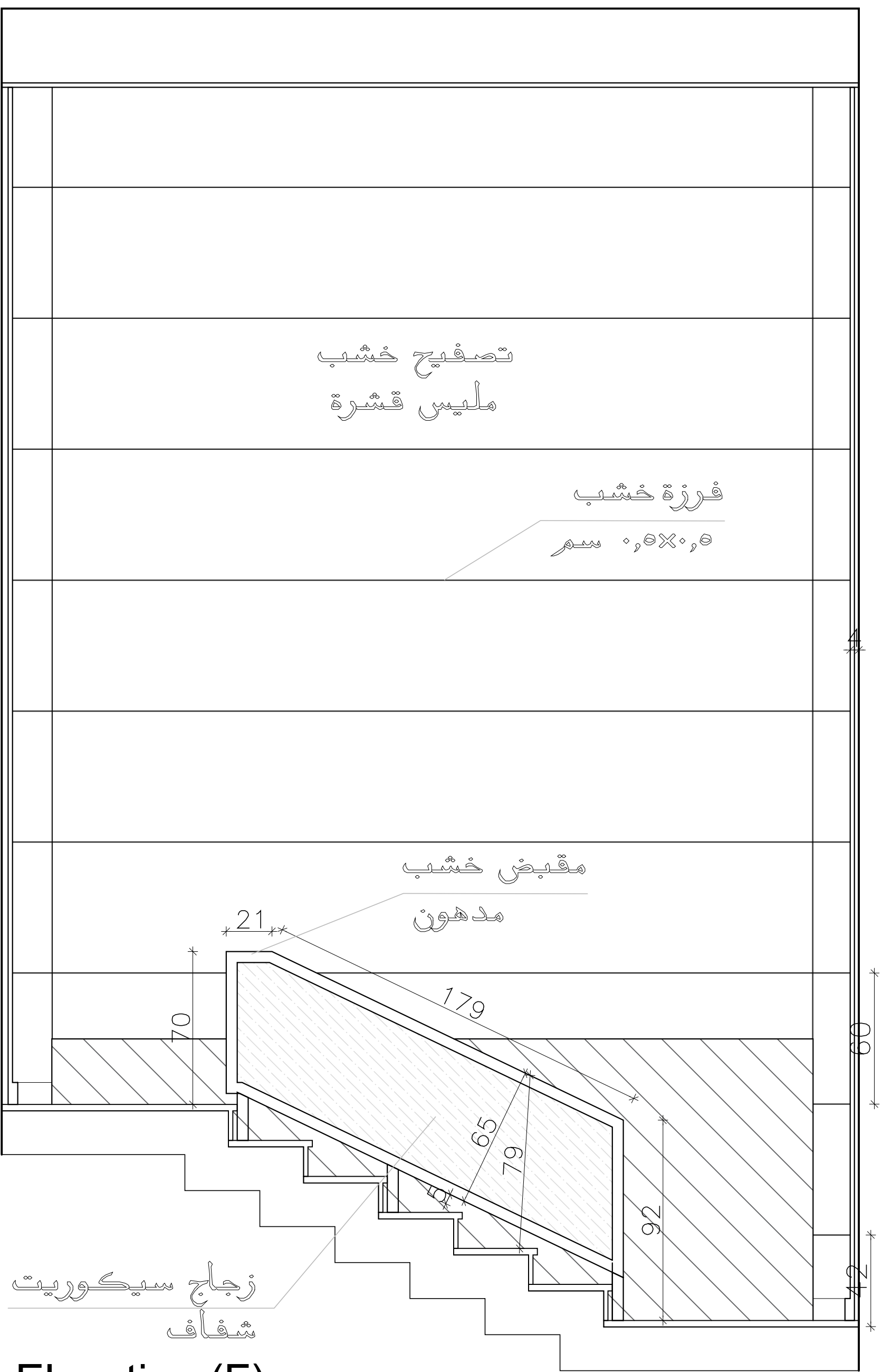
Elevation (F)
